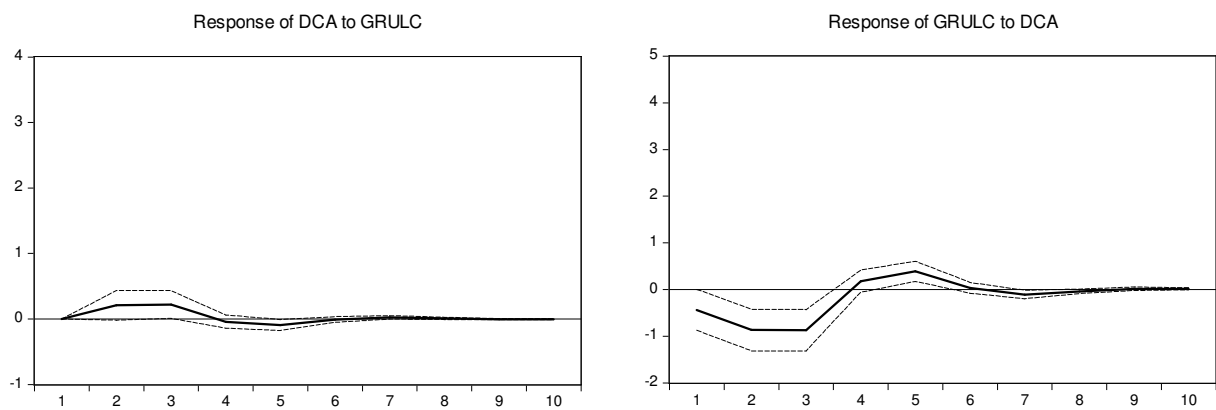
(c) Cholesky decomposition, only contemporary effects from DCA to GRULC
